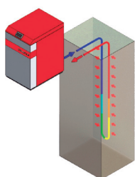
Sondeo vertical
